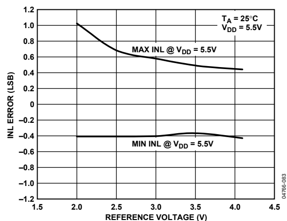
Figure 27. INL vs. V_{REF} @ V_{DD} = 5.5V
