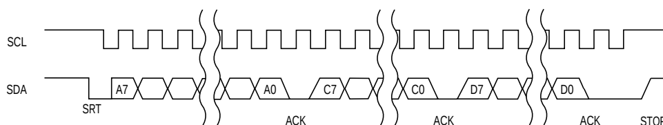
Figure 3. 2-Wire Serial-Interface Timing Diagram ("WriteByte")
