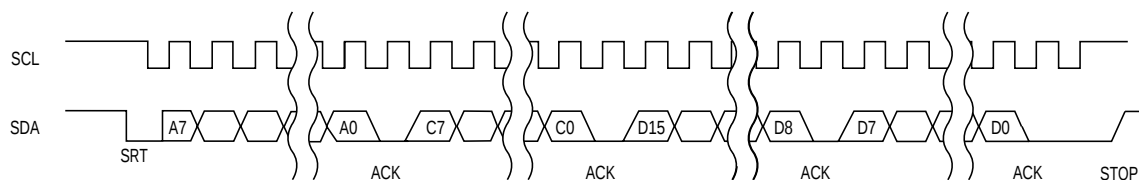
Figure 4. 2-Wire Serial-Interface Timing Diagram ("WriteWord")
