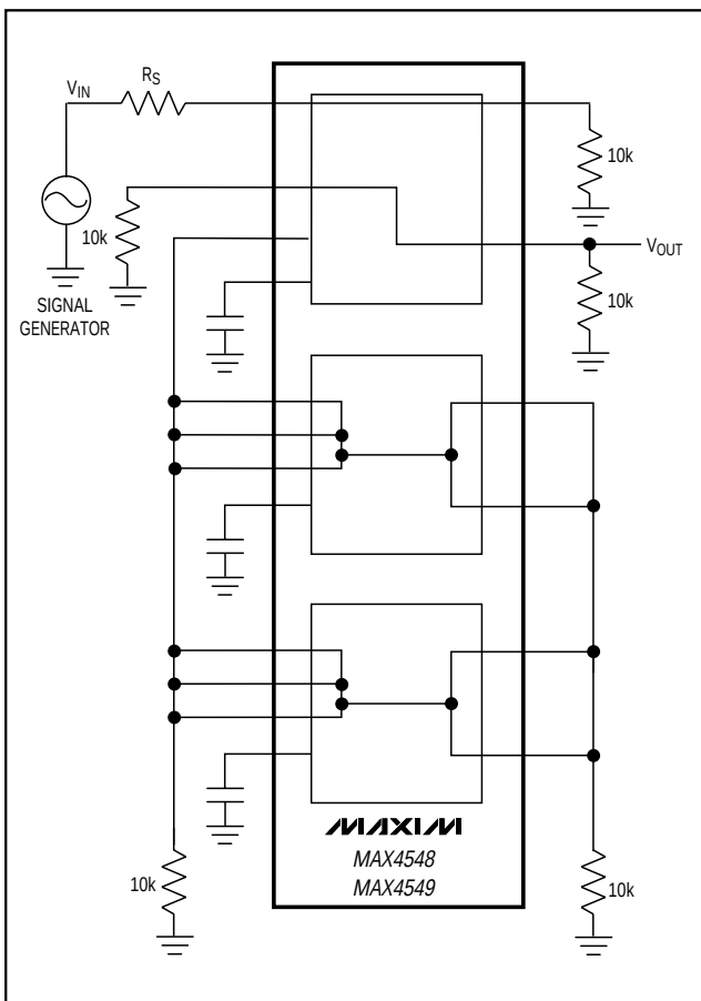
Figure 2b. Crosstalk
