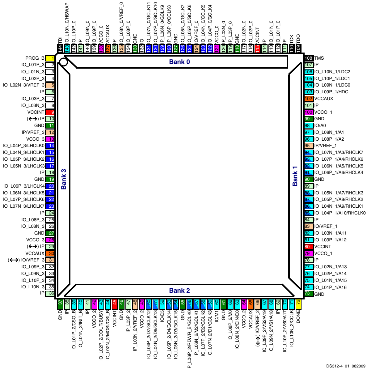
Figure 82: TQ144 Package Footprint (top view)
