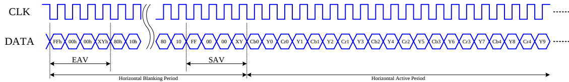
TIMING DIAGRAM OF BT.656 FORMAT FOR DIGITAL VIDEO INPUT
