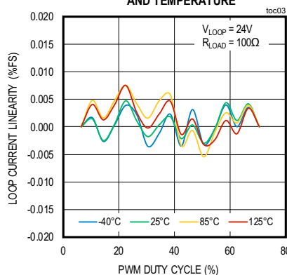
4-20mA LINEARITY vs. PWM DUTY CYCLE AND TEMPERATURE
