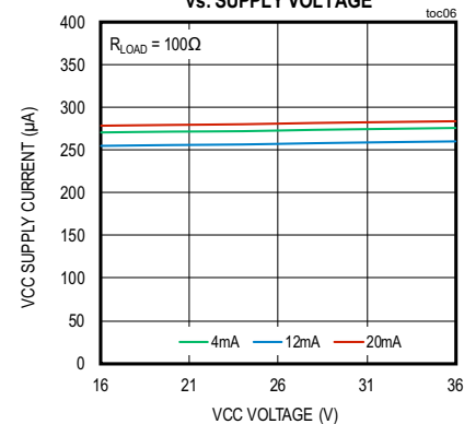
VCC SUPPLY CURRENT vs. SUPPLY VOLTAGE
