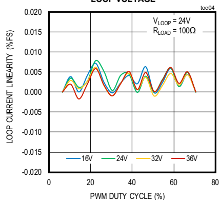
4-20mA LINEARITY vs. PWM DUTY CYCLE AND LOOP VOLTAGE
