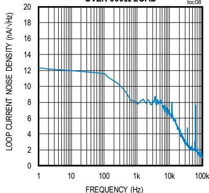
4mA LOOP CURRENT NOISE DENSITY vs. FREQUENCY OVER 500 \Omega LOAD
