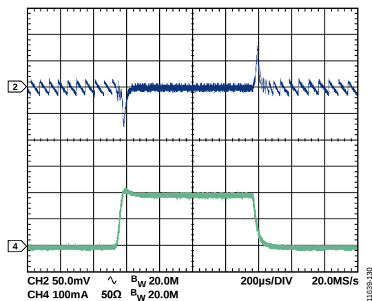
Figure 26. Channel 4 Load Transient, V_{OUT} = 3.3\text{ V} , Auto PSM Mode
