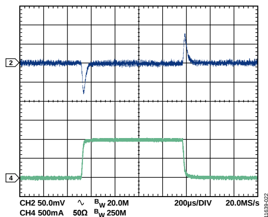
Figure 27. Channel 5 Load Transient, V_{OUT} = 3.3\text{ V} , PPWM Mode
