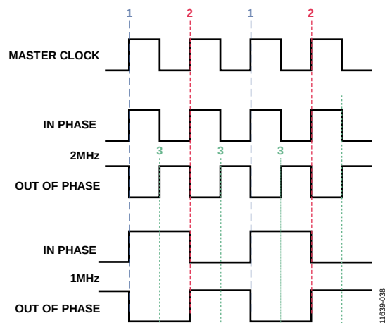
Figure 46. Switching Phase Relationships
