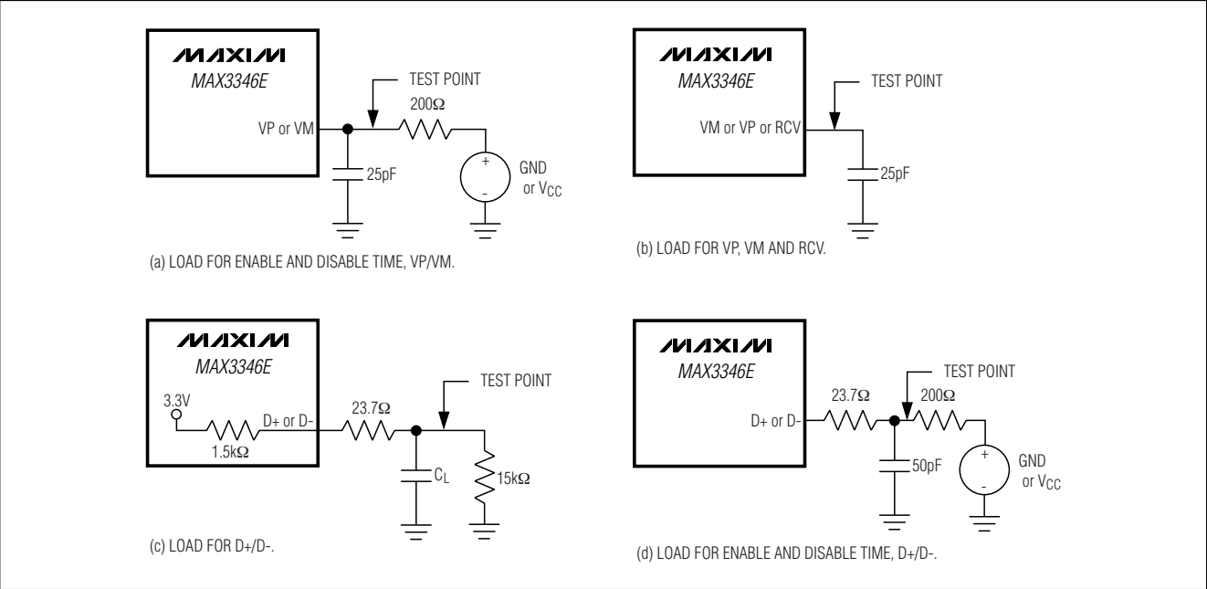
Figure 4. Test Circuits
