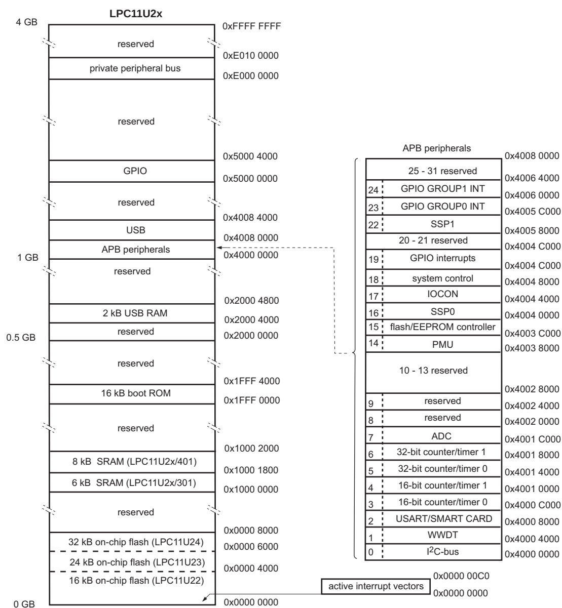
Fig 6. LPC11U2x memory map
