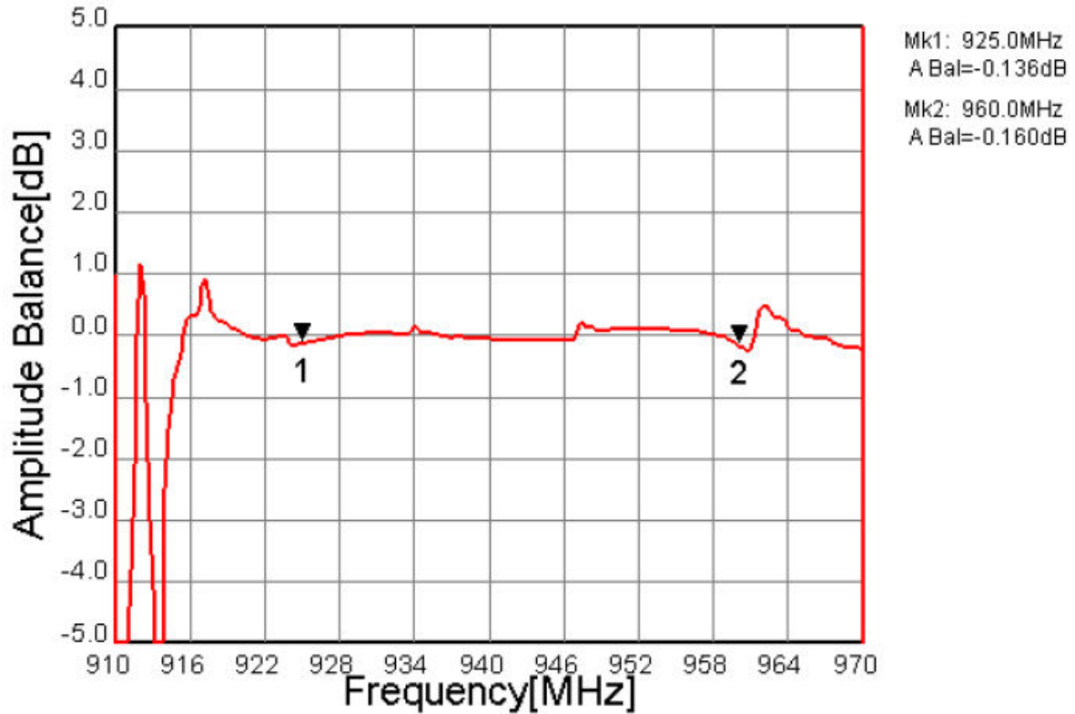
Fig.7 Amplitude Balance
