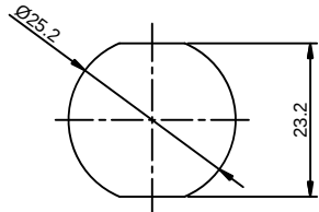
MOUNTING HOLE
