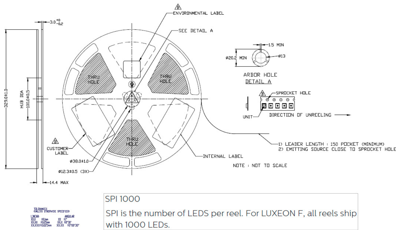
Figure 55. Emitter reel packaging.
