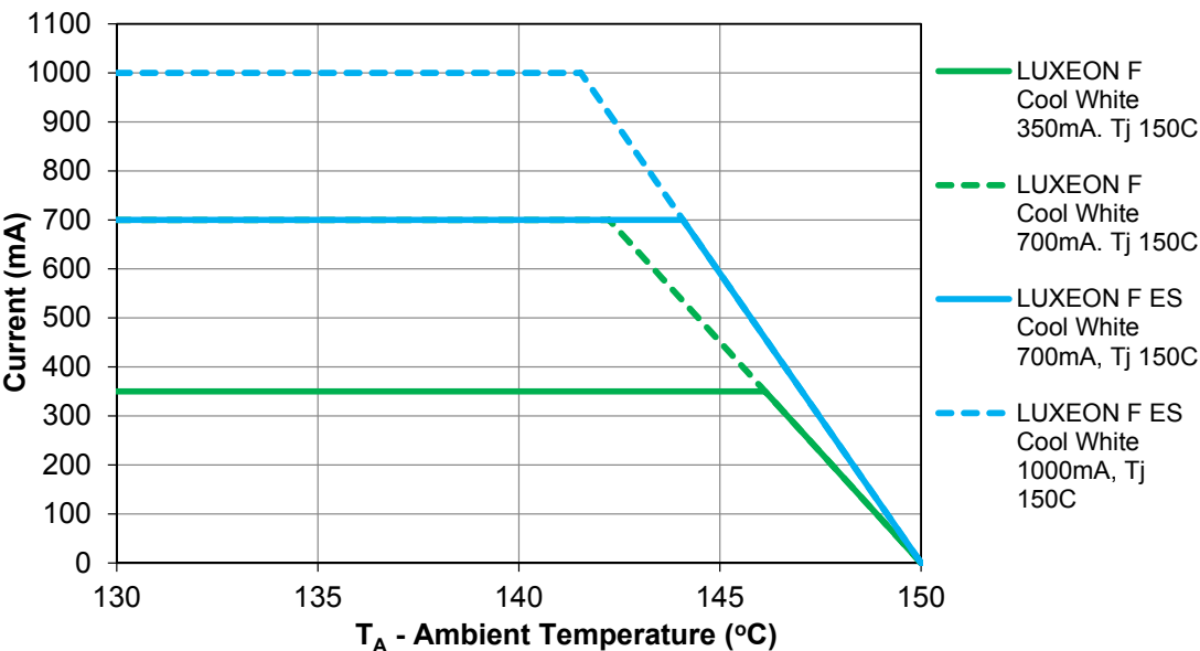
Figure 48. LUXEON F Cool White & ES Cool White Maximum forward current vs Ambient Temperature. Mounting Thermal resistance (case to heat sink – K/W) is not included [1] [2] .
