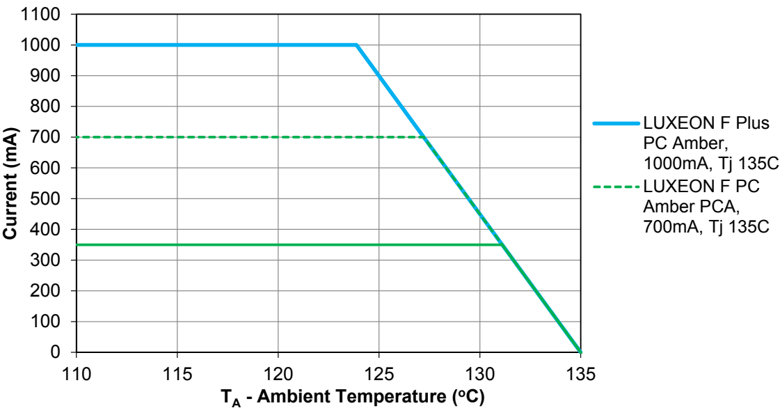
Figure 47. LUXEON F PC Amber & Plus PC Amber Maximum forward current vs Ambient Temperature. Mounting Thermal resistance (case to heat sink – K/W) is not included [1] [2] .
