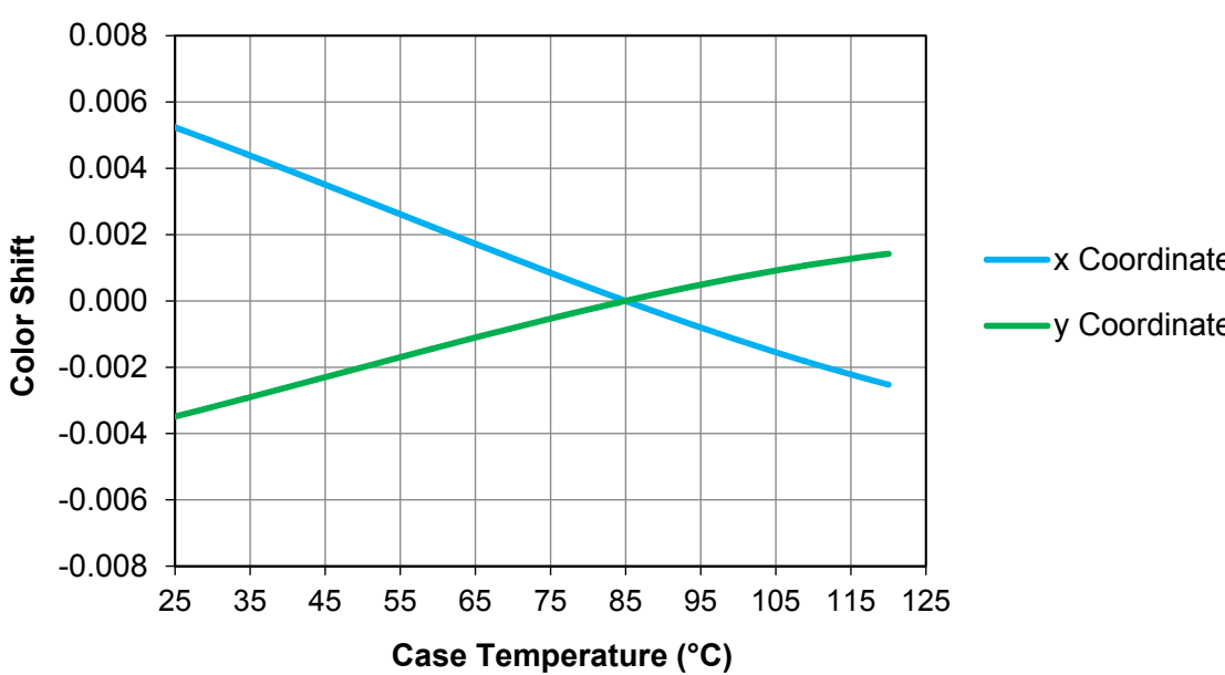
Figure 44. LUXEON F Plus PC Amber color shift range in CIE1931 y coordinate, DC at 1000mA.
