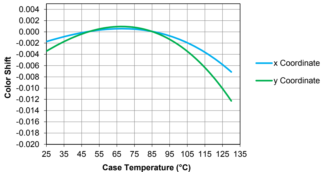
Figure 45. LUXEON F Plus Cool White color shift range in CIE1931 y coordinate, DC at 1000mA.
