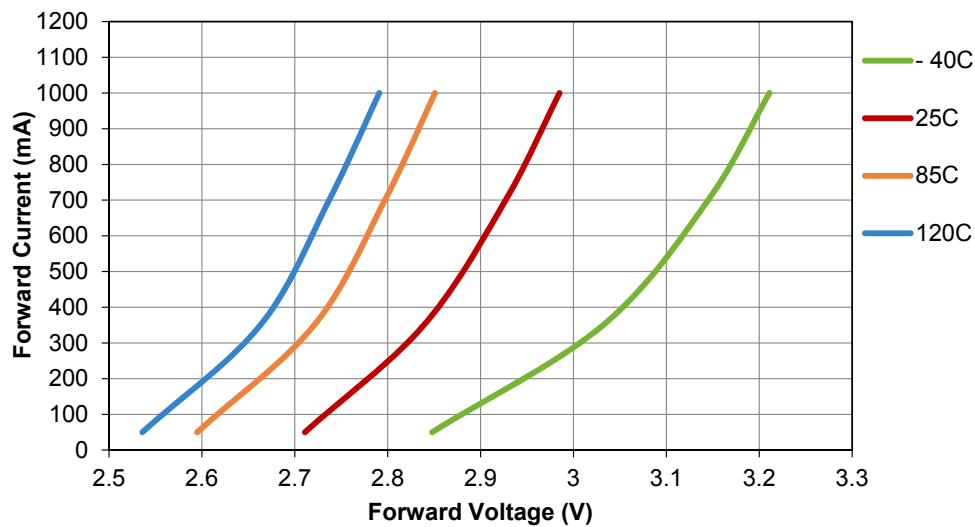
Figure 24. LUXEON F ES Cool White forward current vs. forward voltage MP [1] .
