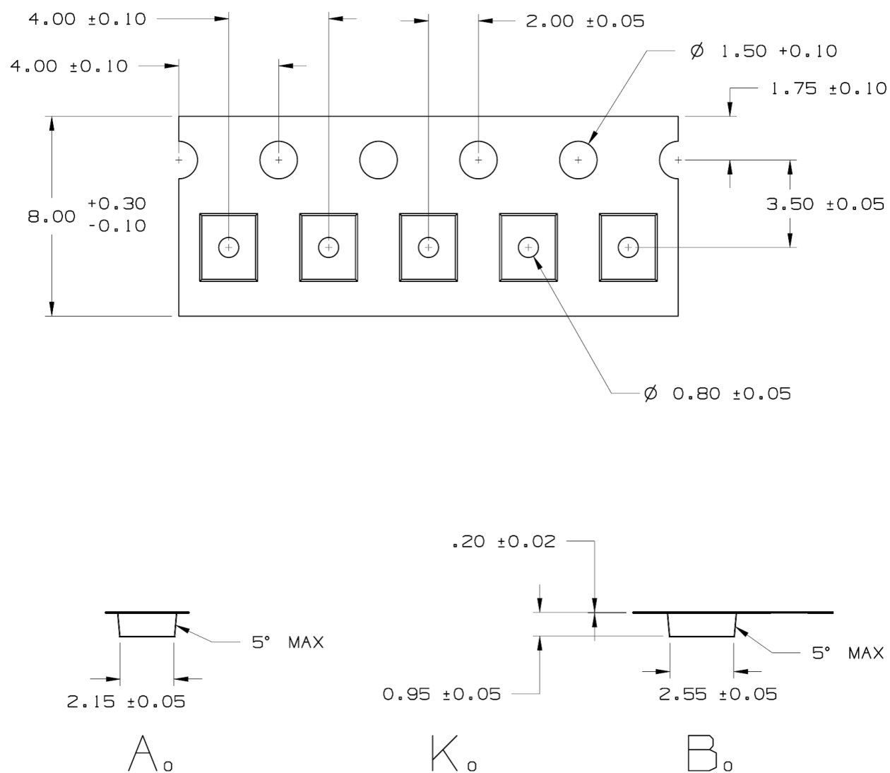
Figure 54. Emitter pocket tape packaging.
