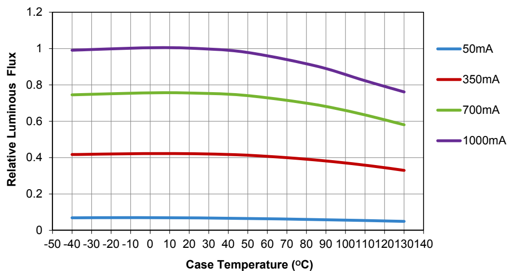
Figure 16. Relative luminous flux vs. case temperature LUXEON F Plus Cool White MP [1] .
