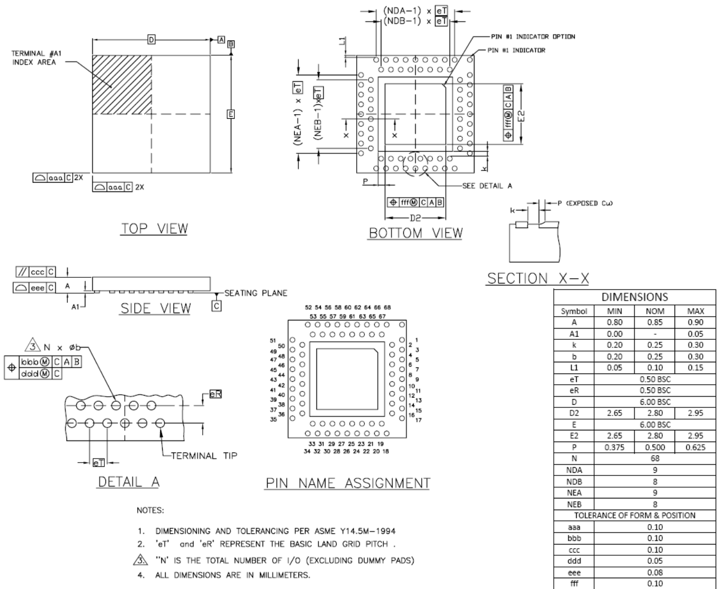
Figure 35. Package Outline
