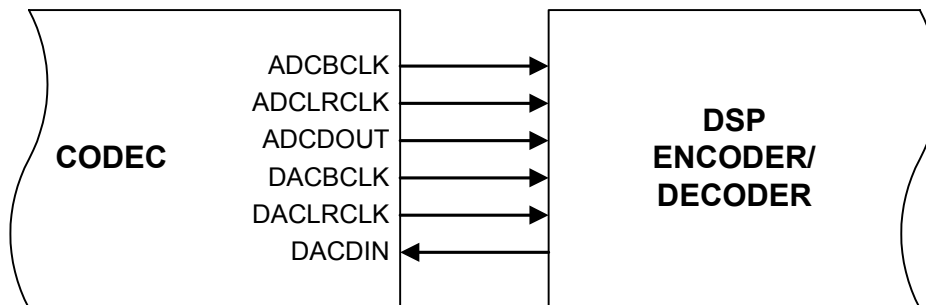
Figure 17. Master mode
