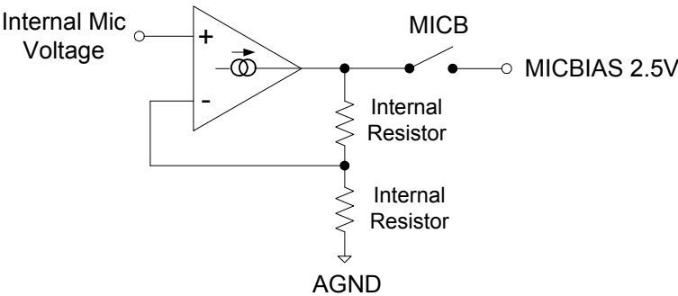
Figure 13. Mic Bias
