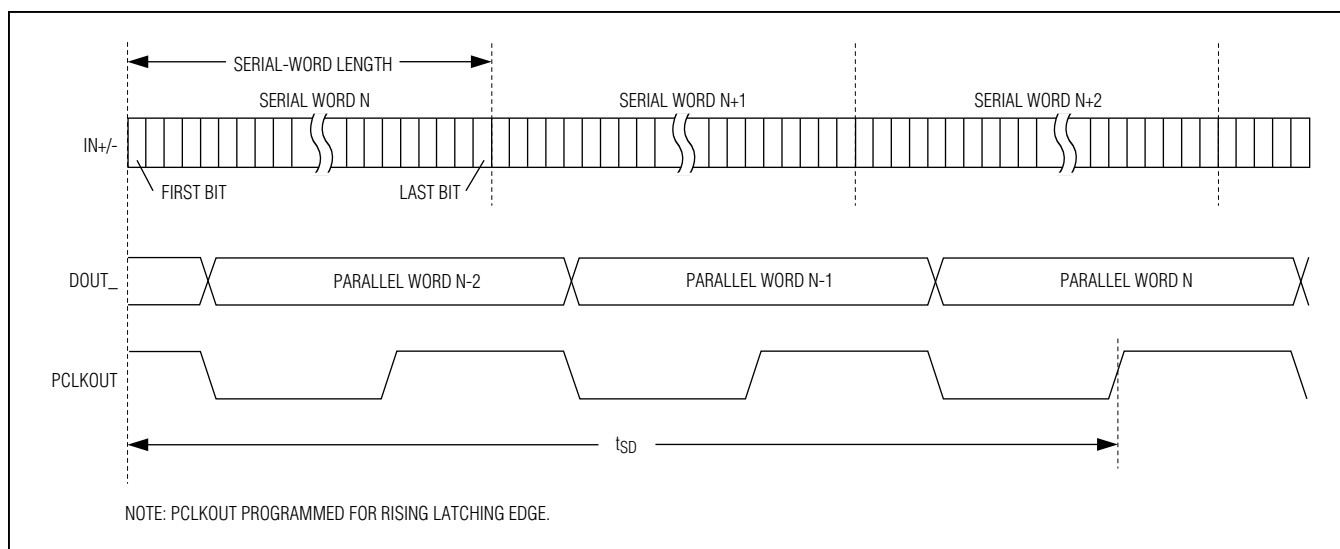
Figure 8. Deserializer Delay
