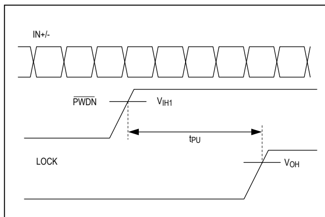
Figure 11. Power-Up Delay
