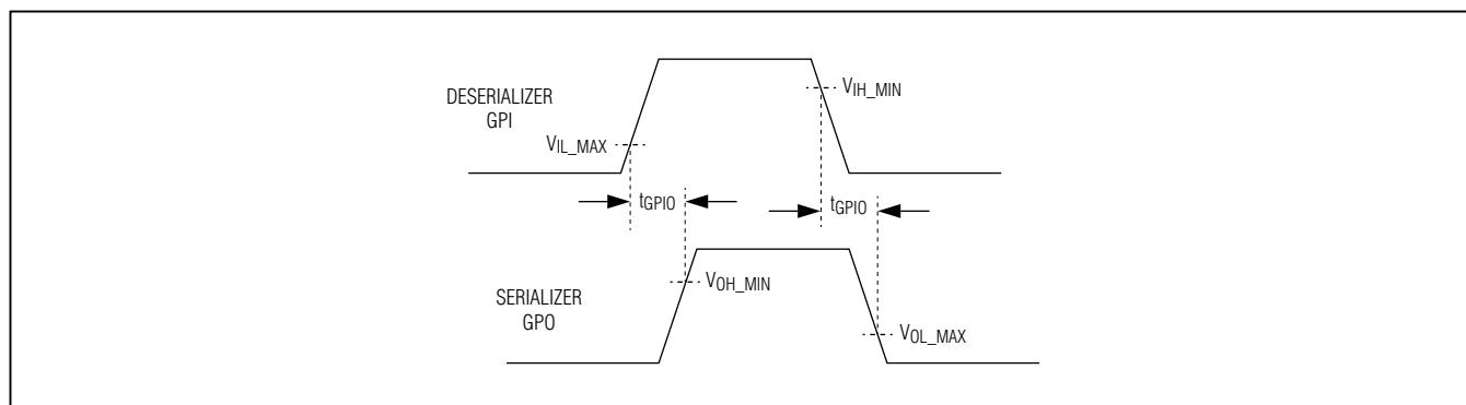
Figure 9. GPI-to-GPO Delay
