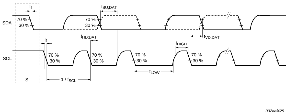
Fig 20. I 2 C-bus pins clock timing
