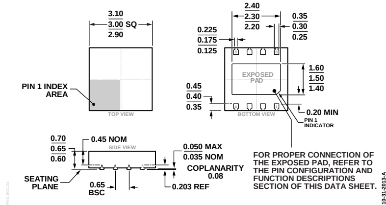
Figure 18. 8-Lead Lead Frame Chip Scale Package [LFCSP] 3 mm x 3 mm Body and 0.65 mm Package Height (CP-8-22) Dimensions shown in millimeters
