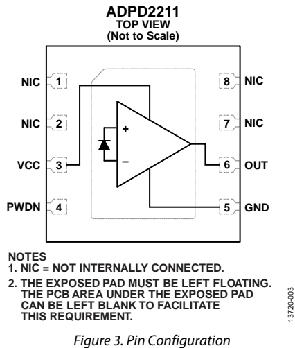
Figure 3. Pin Configuration
