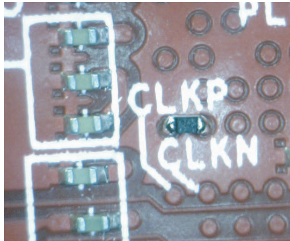
Figure 15. TSW3100 FPGA Clock 100- \Omega LVDS Termination at Pins T31 and T32 of the FPGA
