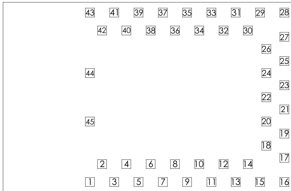
Figure 2 - R41Z Pin out (Top View)
