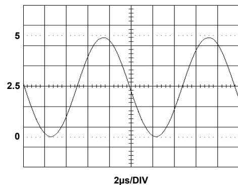
FIGURE 26. OUTPUT SWING
