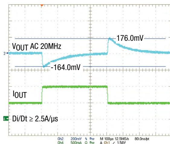
Figure 9. 12V IN , 5.0V OUT Transient Response, 0.5A to 1.0A
