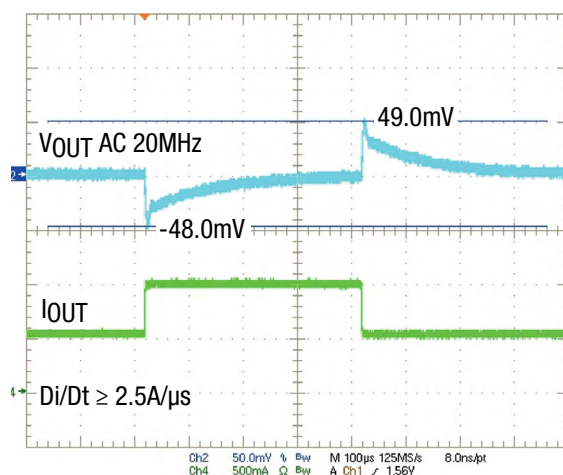
Figure 11. 12V IN , 1.8V OUT Transient Response, 0.5A to 1.0A
