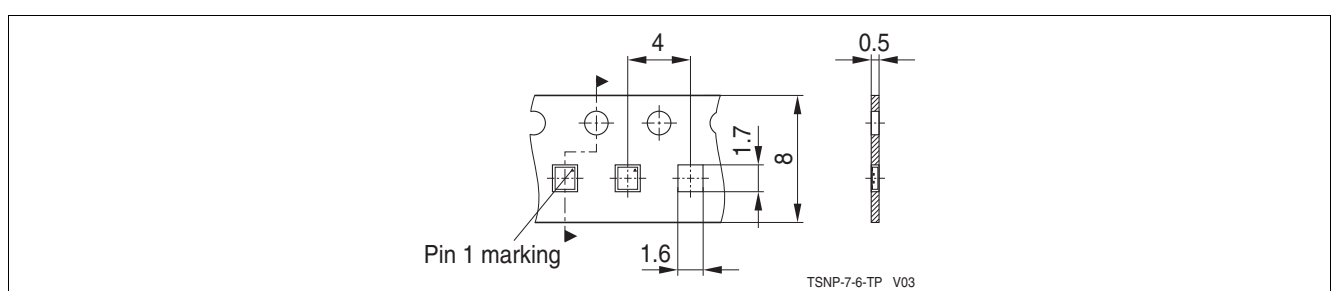
Figure 9-4 Tape Dimensions
