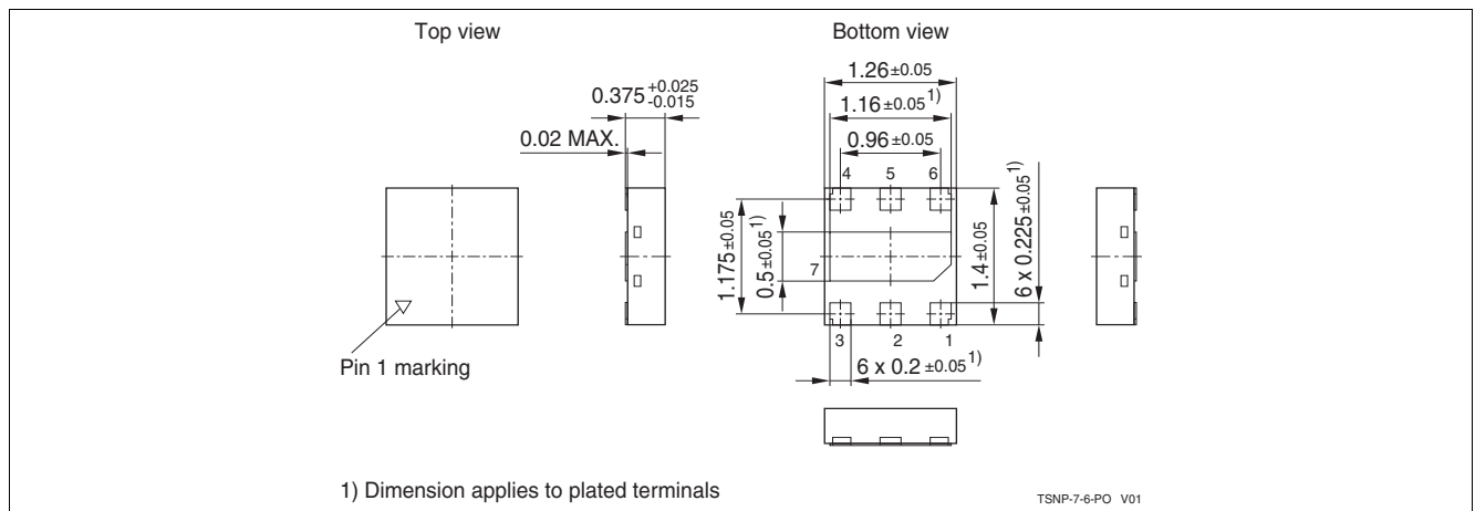
Figure 9-1 Package Outline
