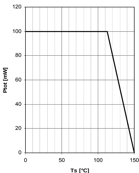
Figure 6-1 Total Power Dissipation P_{tot} = f(T_s)
