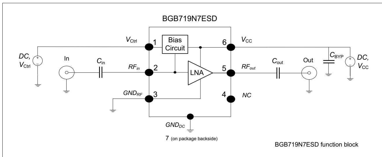
Figure 4-1 Functional Block Diagram
