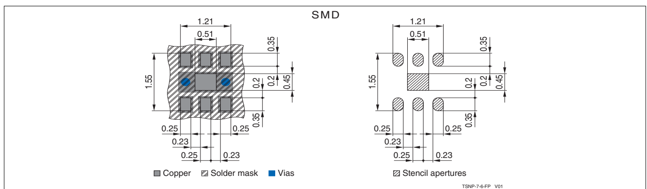
Figure 9-2 Package Footprint
