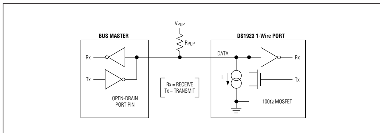
Figure 10. Hardware Configuration
