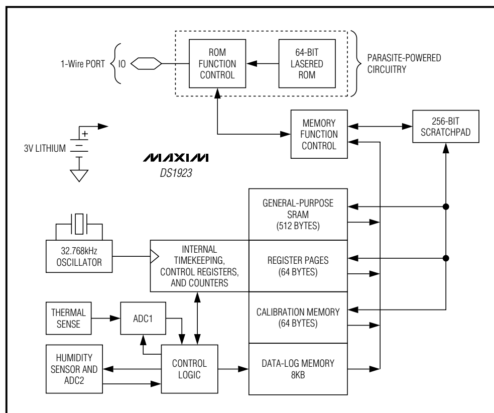
Figure 1. Block Diagram
