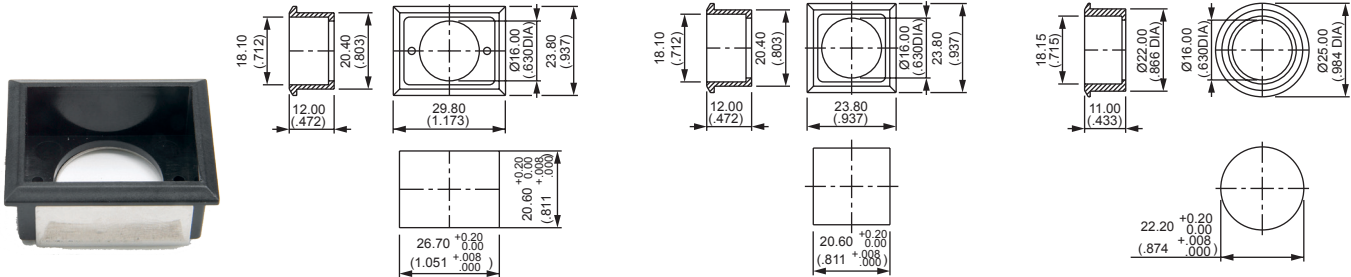
Rectangular : A01FM1
