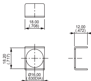
Square : A01MG
