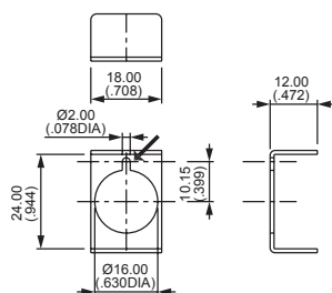
Rectangular : A01MG1
