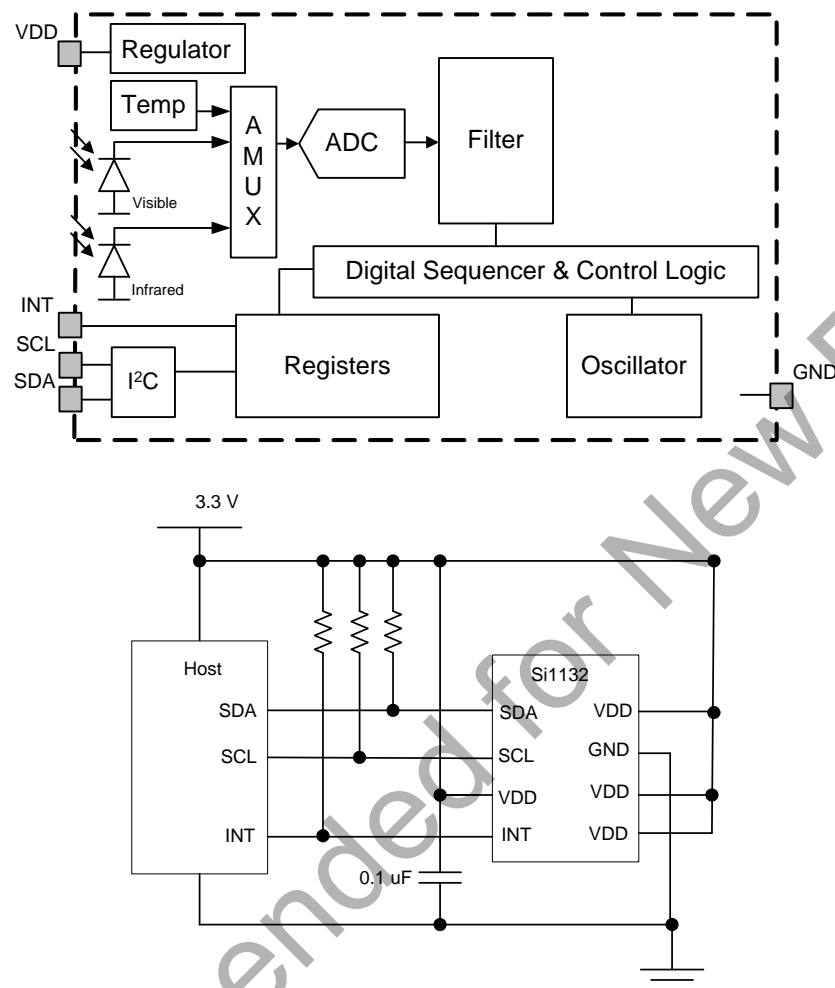
Figure 1. Si1132 Application
