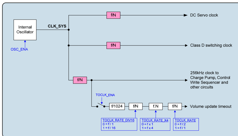
Figure 6 Clocking Scheme
