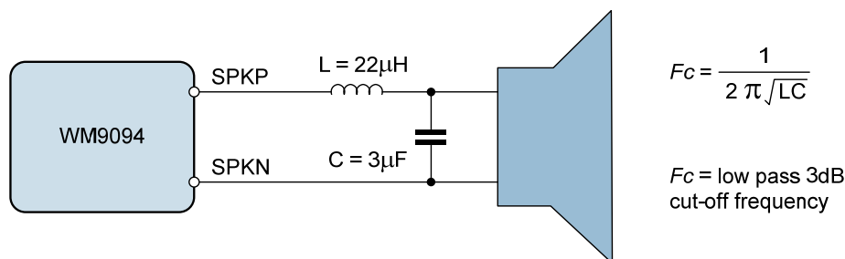
Figure 18 Class D Output Filter Components
