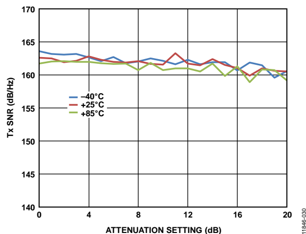
Figure 30. Tx Signal-to-Noise Ratio (SNR) vs. Transmitter Attenuation Setting, GSM Signal of Interest with Noise Measured at 20 MHz Offset
