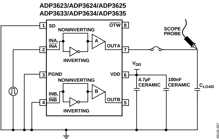
Figure 20. Test Circuit
