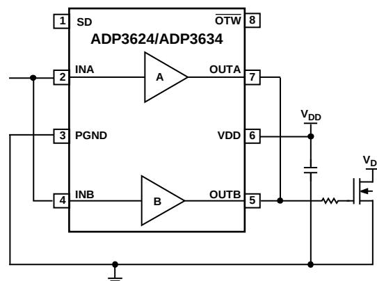
Figure 25. Parallel Operation
