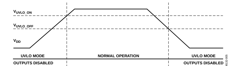
Figure 5. UVLO Function
