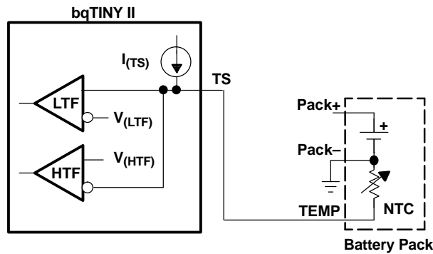
Figure 28. TS Pin Configuration
