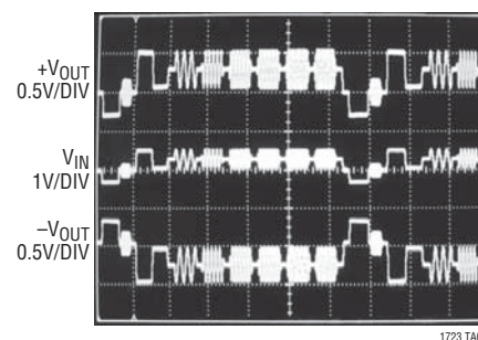
Line Driver Multiburst Video Signal
