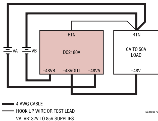
Figure 1. Test Setup
