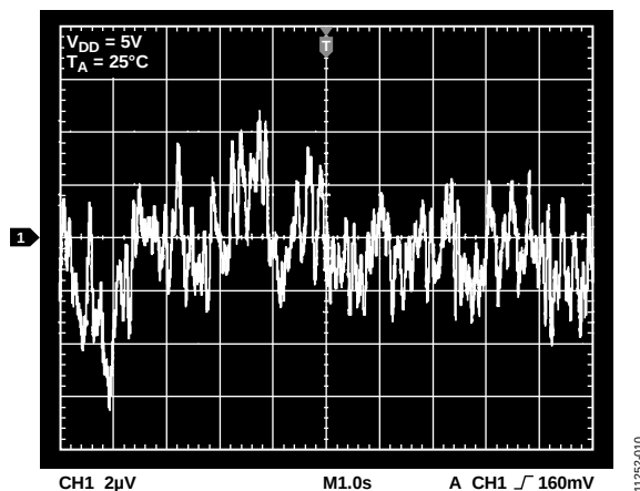
Figure 8. Internal Reference Noise, 0.1 Hz to 10 Hz
