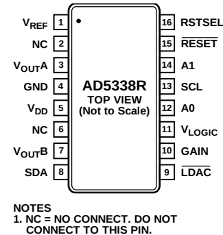
Figure 4. 16-Lead TSSOP Pin Configuration
