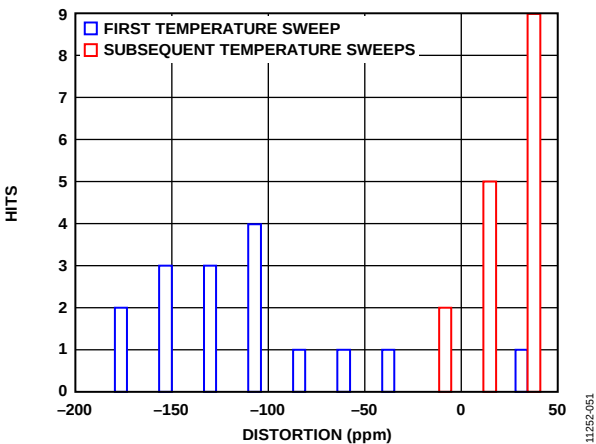
Figure 49. Thermal Hysteresis
