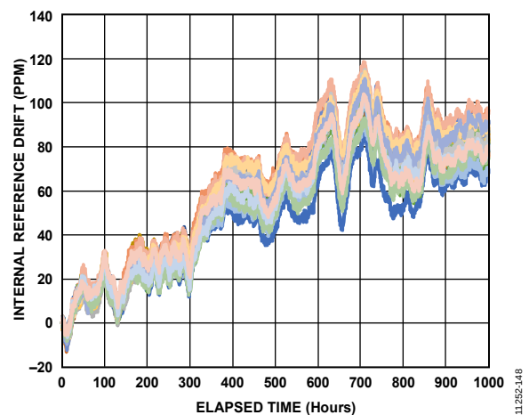
Figure 48. Reference Drift Through to 1000 Hours
