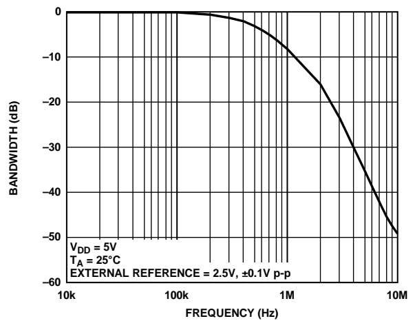
Figure 39. Multiplying Bandwidth, External Reference = 2.5 V, ±0.1 V p-p, 10 kHz to 10 MHz
