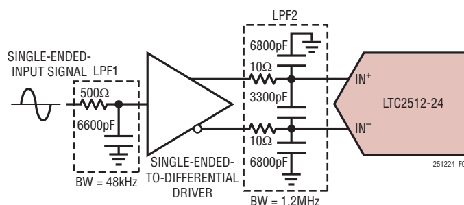
Figure 4. Filtering Input Signal
