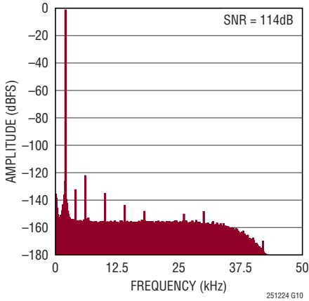
128k Point FFT f_{\text{SMPL}} = 1.6\text{Msps} , f_{\text{IN}} = 2\text{kHz} , DF = 16
