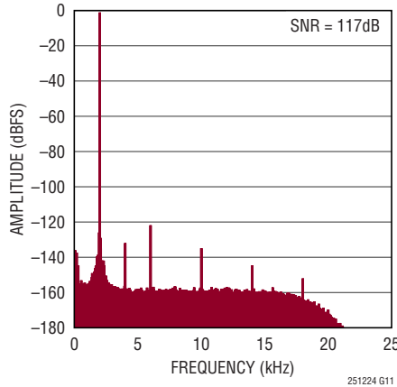
128k Point FFT f_{\text{SMPL}} = 1.6\text{Msps} , f_{\text{IN}} = 2\text{kHz} , DF = 32
