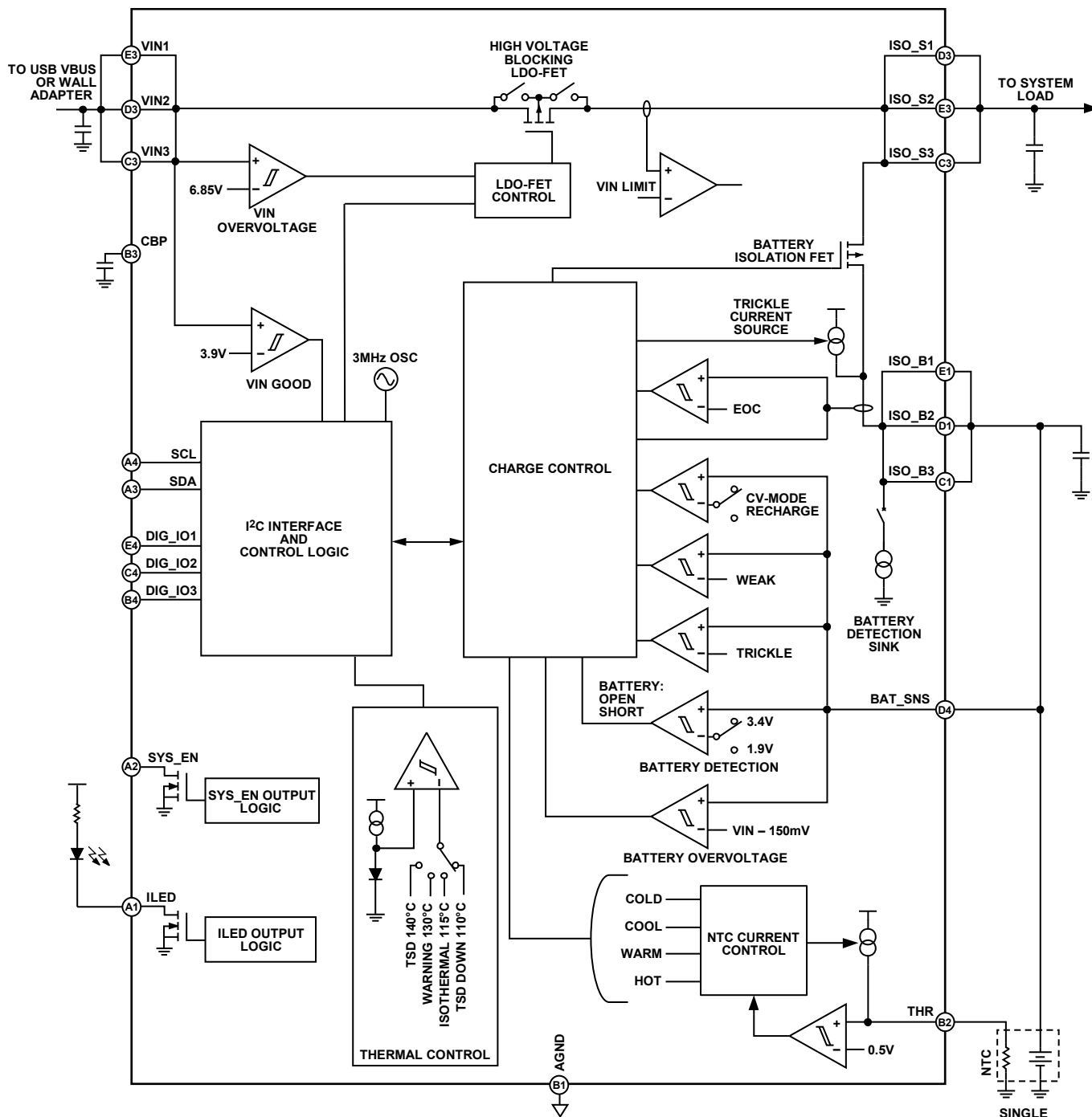
Figure 29. Block Diagram
