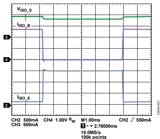
Figure 27. Load Transient. I_{\text{ISO\_sx}} Load = 300 mA to 1500 mA to 300 mA, \text{EN\_CHG} = \text{High} , \text{ILIM}[3:0] = 0110 (Binary) = 500 mA
