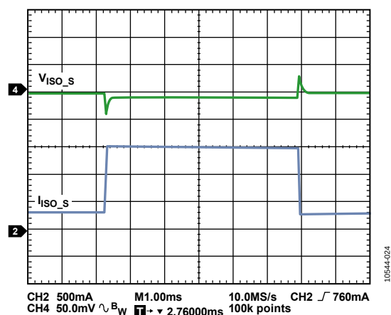
Figure 24. Load Transient, I_{\text{ISO\_sx}} Load = 300 mA to 1500 mA to 300 mA
