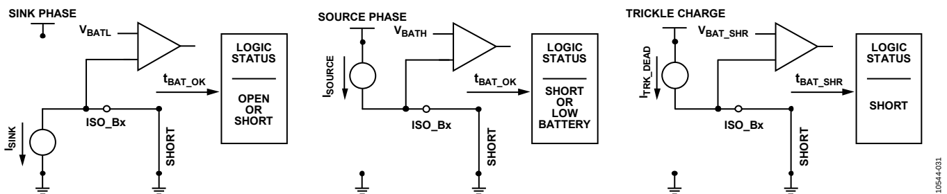
Figure 31. Trickle Charge
