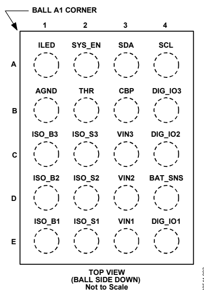
Figure 3. Pin Configuration
