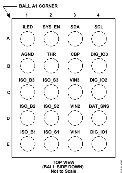
Figure 3. Pin Configuration
