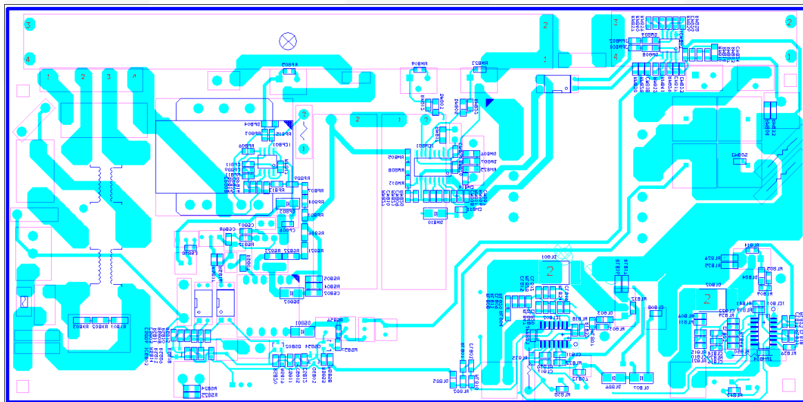
Figure 8. Bottom Pattern
