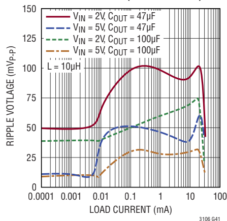
3.3V Output Voltage Ripple vs Load Current ( I_{LIMSEL} Low)
