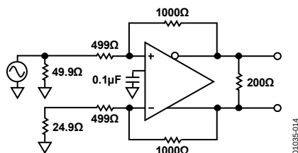
Figure 57. Basic Test Circuit, G = +2
