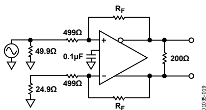
Figure 58. Test Circuit for Various Gains
