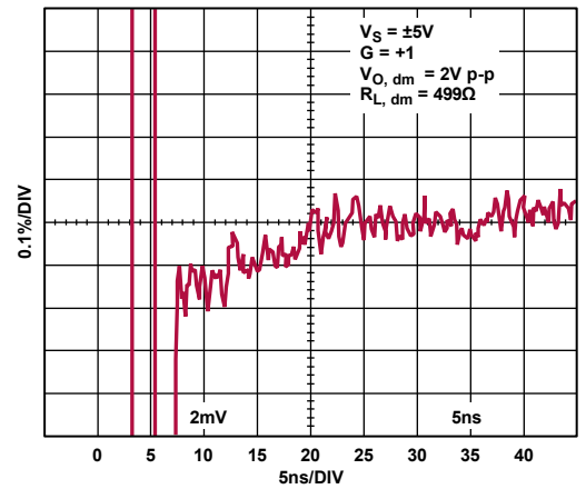
Figure 44. 0.1% Settling Time
