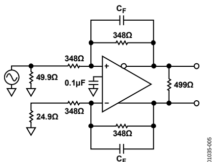
Figure 56. Basic Test Circuit, G = +1
