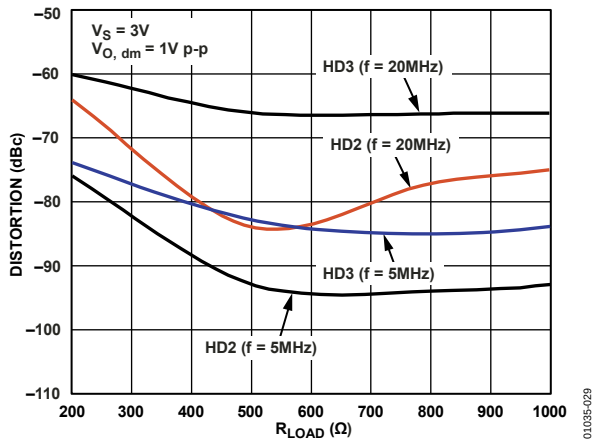
Figure 24. Harmonic Distortion vs. R_{LOAD} , G = +1 (See Figure 62)
