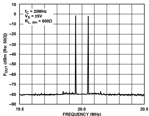
Figure 33. Intermodulation Distortion, G = +1
