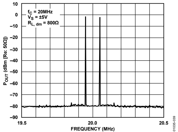
Figure 33. Intermodulation Distortion, G = +1
