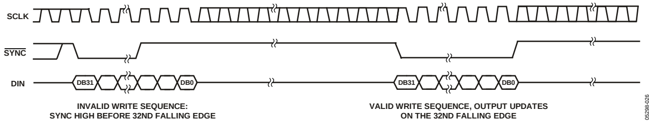
Figure 43. \overline{\text{SYNC}} Interrupt Facility
