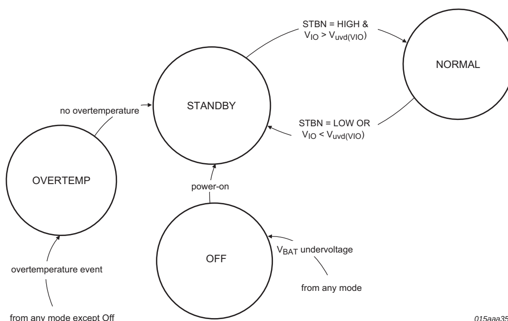
Fig 3. UJA1161 system controller state diagram
