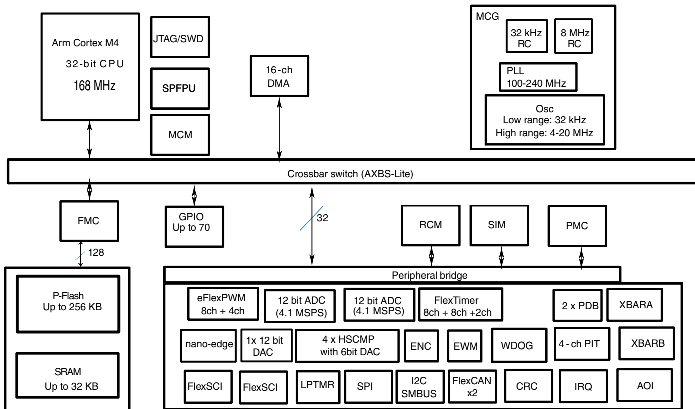
Figure 1. MWCT1x23 block diagram
