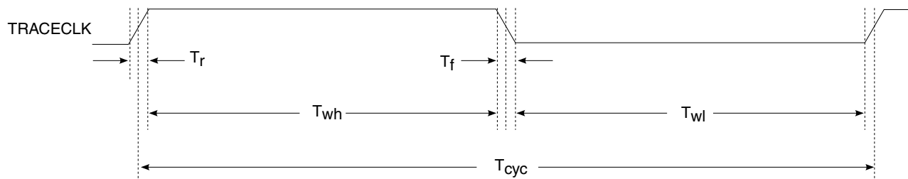
Figure 8. TRACE_CLKOUT specifications
