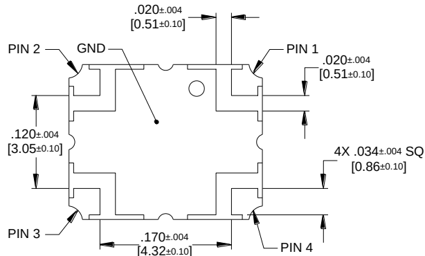
Bottom View (Far-Side)
