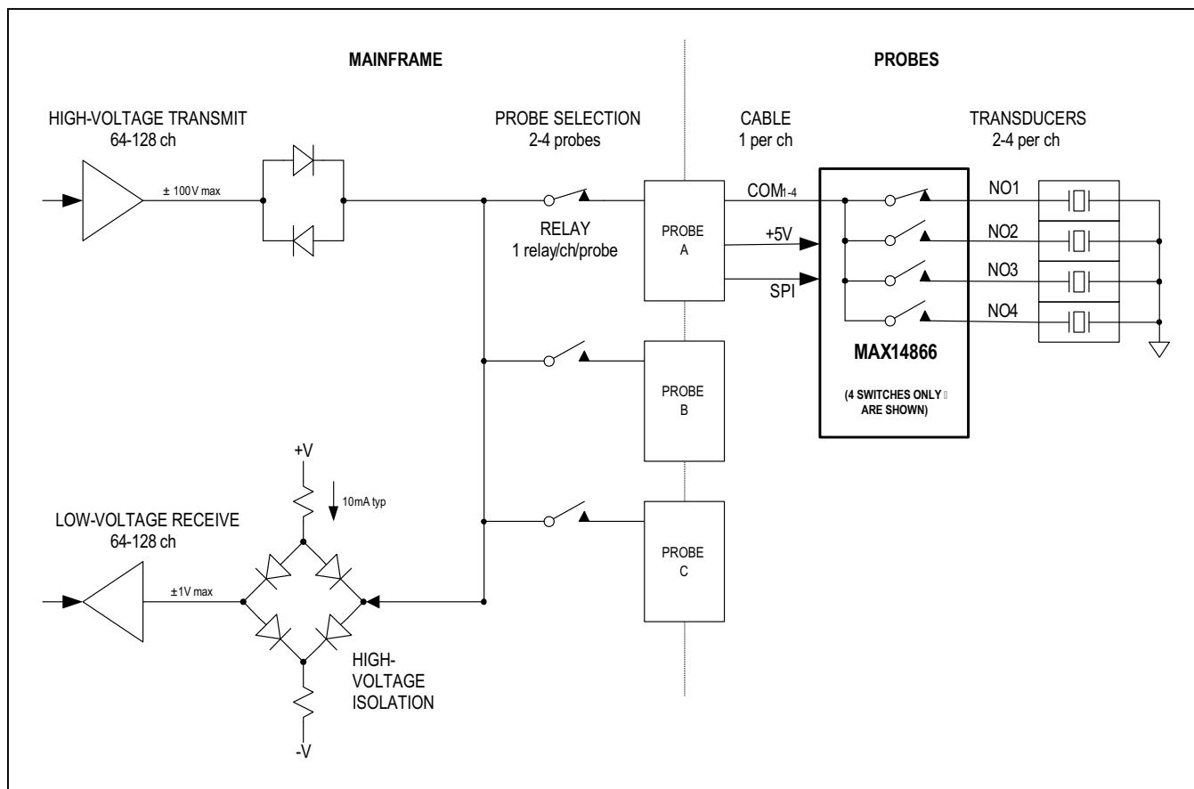
Figure 5. Application Diagram
